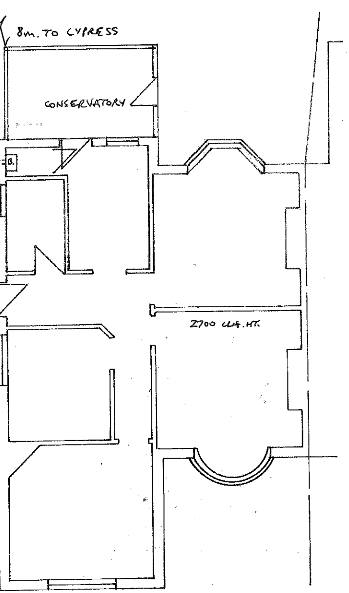
EXISTING PLAN 1:100
