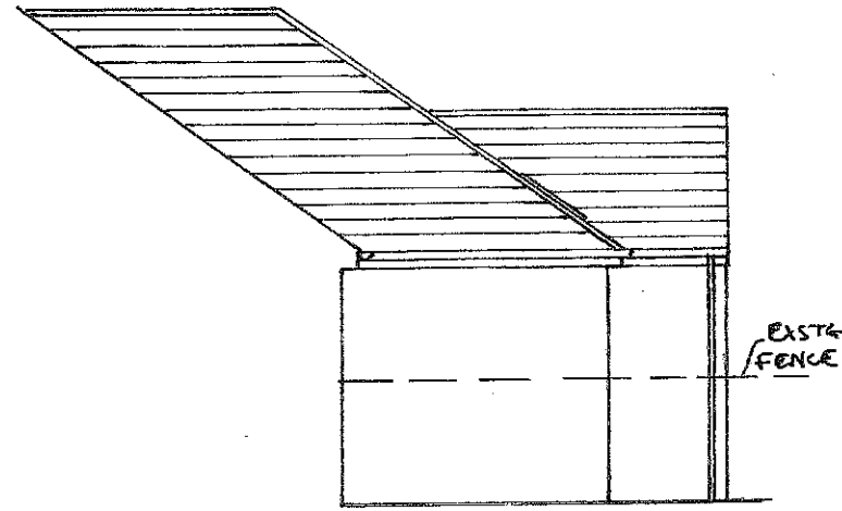
PROPOSED INNER SIDE 1:100
